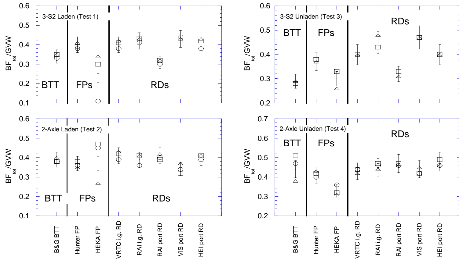
Figure 11. Repeatability of PBBT-reported \text{decel}_{EQ} ( \text{BF}_{TOT}/\text{GVW} ) for weakly braked vehicles (Tests 1 - 4). Data for replicate 1 (○), replicate 2 (□) and replicate 3 (△) are plotted. The error bars represent the acceptable repeatability range for \text{decel}_{EQ} ( \pm 10\% , as listed in Table 5).
