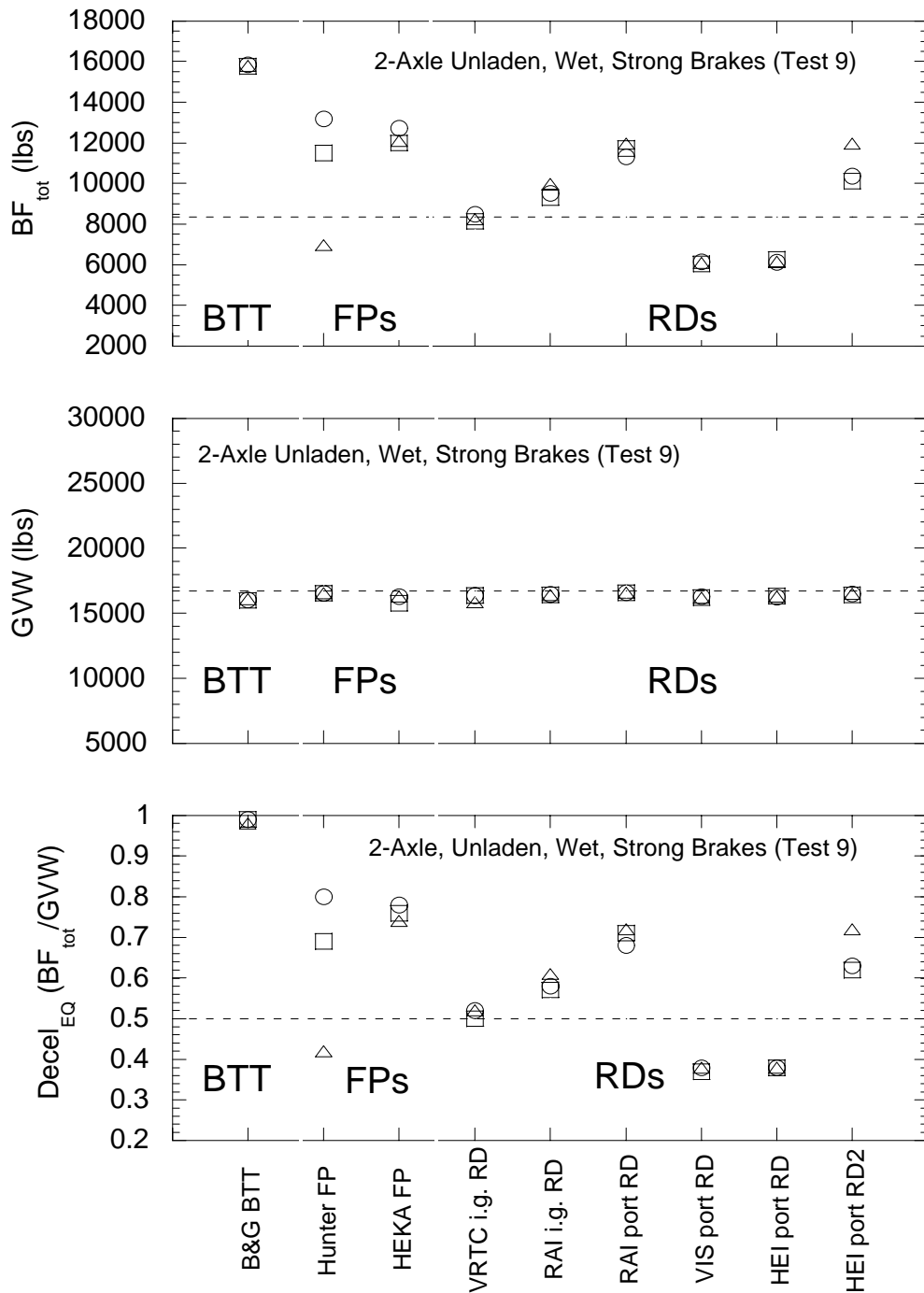
Figure 16. Strongly braked 2-axle vehicle, unladen, wet (Test 9). Data for replicate 1 ( \circ ), replicate 2 ( \square ) and replicate 3 ( \triangle ) are plotted. The dashed lines represent the reference data from 32.2 km/hr (20 mph) on-road stops and certified scale weight measurements.
